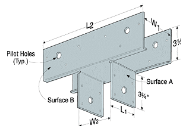
PC/EPC POST CAPS
