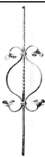
B/500 MAT: 1/2" SQ. H: 36" W: 7-3/32" HWOSINDB/500
