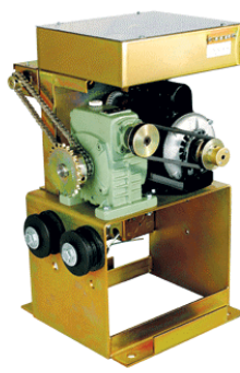
FAIL SECURE MODEL
