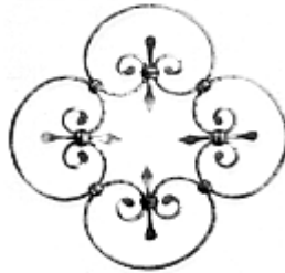
24/2 MAT: 3/8" X 3/16" DIA: 14-15/16" HWOSIND24/2
