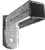
02-180 FMBS-SQ 1" (1/4" HOLE) FITS: 1" SQ. TUBE (16 GA) HOLE: FITS 1/4" FASTENERS FINISH: ZINC PLATED HWOS02-180
