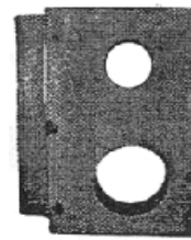
01-172 DOUBLE HOLE FLAT 1-5/16" RIGHT SIDE W: 1-1/2" H: 6-7/8" L: 4-1/4" BACKSET: 2-3/8" BIG HOLE: 2-1/8" SMALL HOLE: 1-1/2" HWOS01-172
