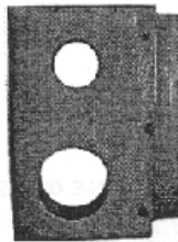
01-171 DOUBLE HOLE FLAT 1-5/16" LEFT SIDE W: 1-1/2" H: 6-7/8" L: 4-1/4" BACKSET: 2-3/8" BIG HOLE: 2-1/8" SMALL HOLE: 1-1/2" HWOS01-171
