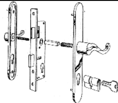
15-SLH123 DELUXE THINLINE LOCKSET SOLID BRASS CYLINDERS DEADBOLT THROW: 5/8" LATCH: 1/2" HWOS15-SLH123
