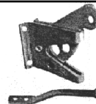
04-158 BIG UNIVERSAL GATE LATCH W/ HOLES & PIN H: 4" L: 2-1/4" FINISH: MILL HWOS04-158
