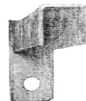
02-172 FMBS-CHANNEL 1" (DOWN) FITS: 1" SQ. TUBE HOLE: FITS 3/8" FINISH: MILL HWOS02-172
