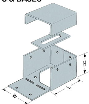
AB/ABA/ABE/ABU ADJUSTABLE AND STANDOFF POST BASES
