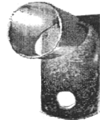
02-152 FMBS-BIAS RD 1-1/8" FITS: 1-3/8" RD. TUBE HOLE: FITS 3/8" FAST. FINISH: ZINC PLATED HWOS02-152
