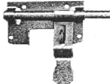
04-171 MEX SLIDE BOLT- 1/2" (Z) H: 2-1/2" W: 4" BOLT: 1/2" RD THROW: 1-7/8" FINISH: ZINC HWOS04-171
