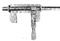
04-175 BIG SLIDE BOLT-5/8" H: 3" W: 6-1/4" BOLT: 5/8" RD THROW: 4-3/4" FINISH: MILL HWOS04-175
