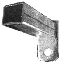
02-151 FMBS-SQ 1" FITS: 1" SQ. TUBE (16 GA) HOLE: FITS 3/8" FASTENERS FINISH: ZINC PLATED HWOS02-151
