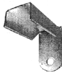
02-155 FMBS-BIAS REC 1-1/2" X 1" FITS: 1-1/2" REC. TUBE HOLE: FITS 3/8" FAST. FINISH: ZINC PLATED HWOS02-155
