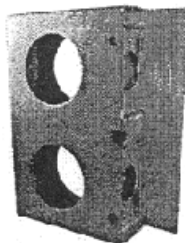
01-169 DOUBLE HOLE FLAT 1-1/2" W: 1-1/2" H: 3-1/2" L: 4-1/2" BACKSET: 2-3/4" HOLE: 2-1/8" HWOS01-169
