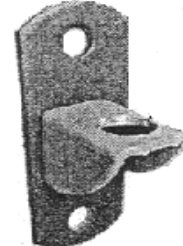
02-359 BASE PLATE HINGE HINGE HOLE: 1/2" RD MTL. SCREW HOLE: FITS 3/8" W: 1-1/2" H: 3-1/2" HWOS02-359
