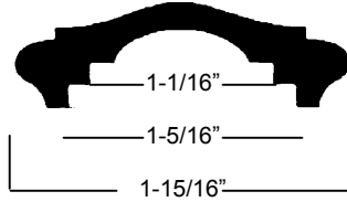
03-301 MOLDED CAP RAIL 1-15/16" FITS OVER 1-1/4" HWOS03-301
