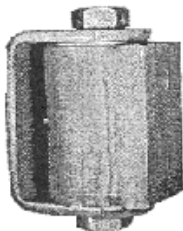
05-052 SMALL (FLAT BASED) H: 3-1/2" W: 1-1/2" GAP: 2-1/2" CAP: 400 lbs. HWOS05-052
