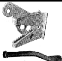
04-161 BIG GATE LATCH NO HOLE H: 3-1/8" L: 2-3/4" B: 1-5/16" FINISH: MILL HWOS04-161
