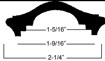
03-303 MOLDED CAP RAIL 2-1/4" FITS OVER 1-1/2" HWOS03-303
