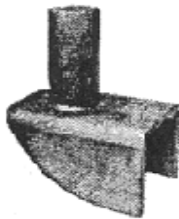
02-235 BATWING MALE W: 1" L: 2" PIN: 1/2" HWOS02-235
