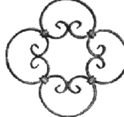
24/C/1 MAT: 1/2" X 1/4" DIA: 14-15/16" HWOSIND24/C/1
